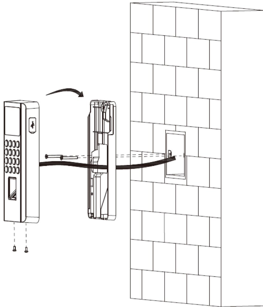
Figure 2-8 86 box mount
