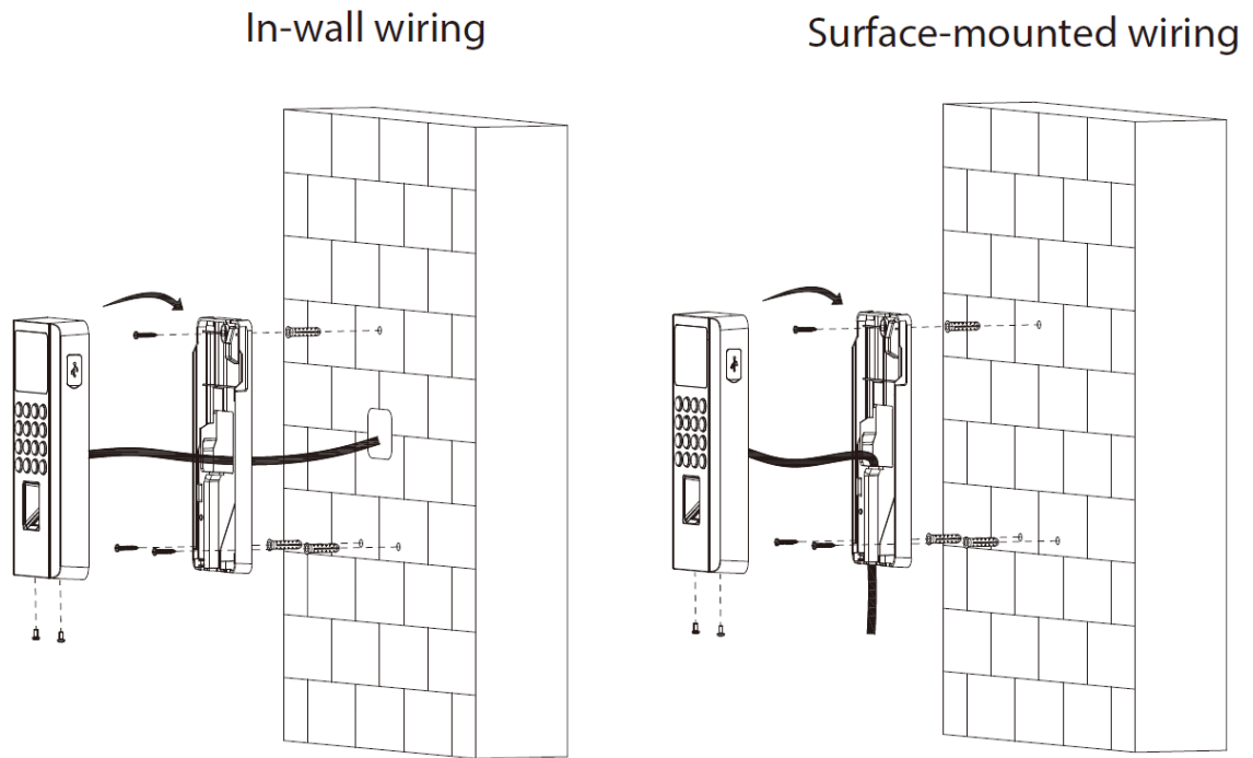
Figure 2-7 Wall mount
